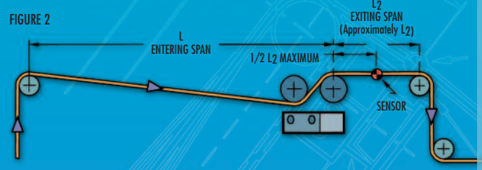
Typical Straight-Through Threading (S-Wrap)
