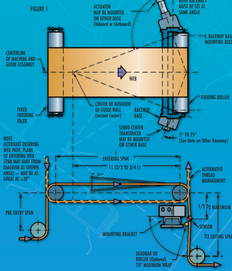
Typical Straight-Through Threading (S-Wrap)
